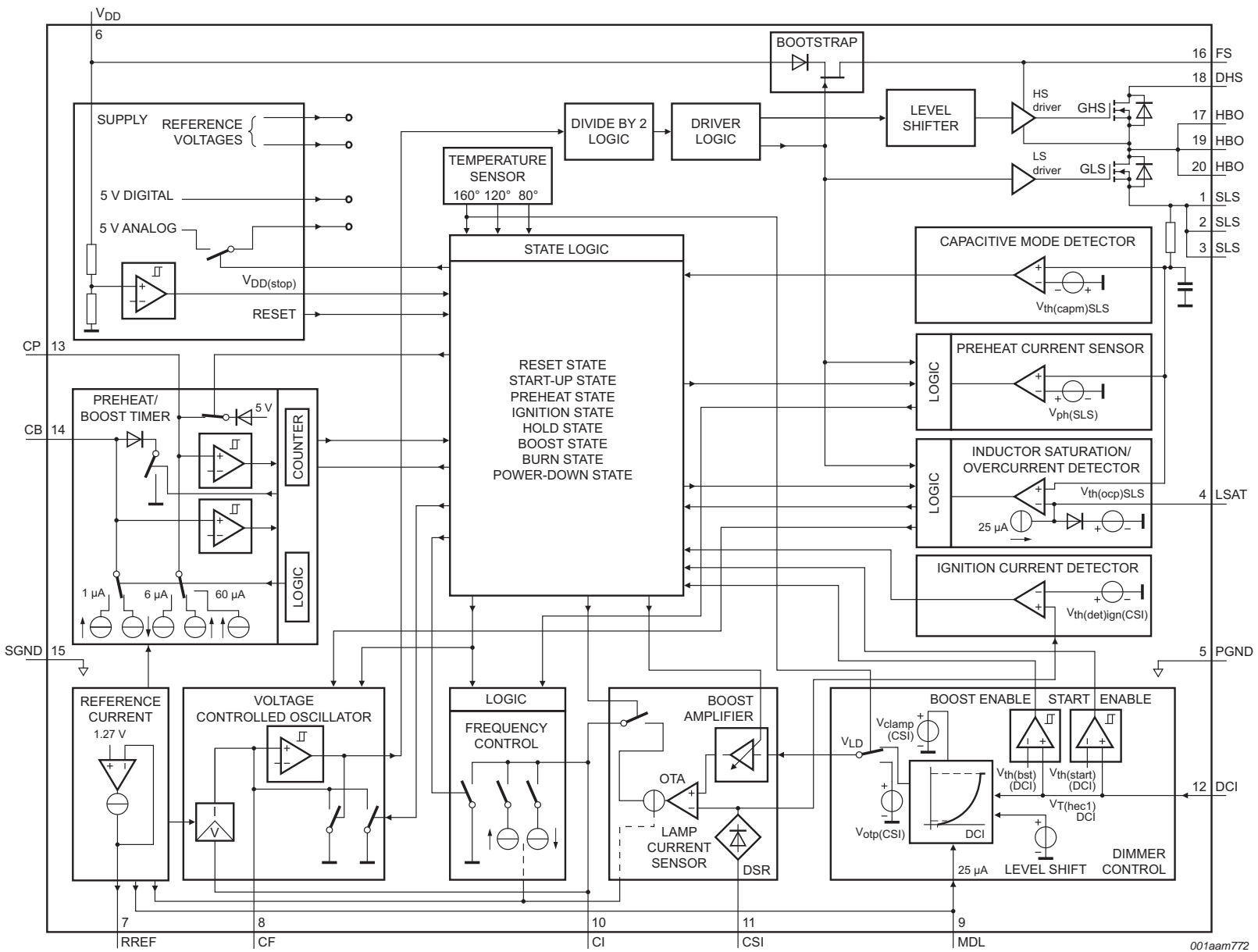
Fig 1. Block diagram UBA20271/2
