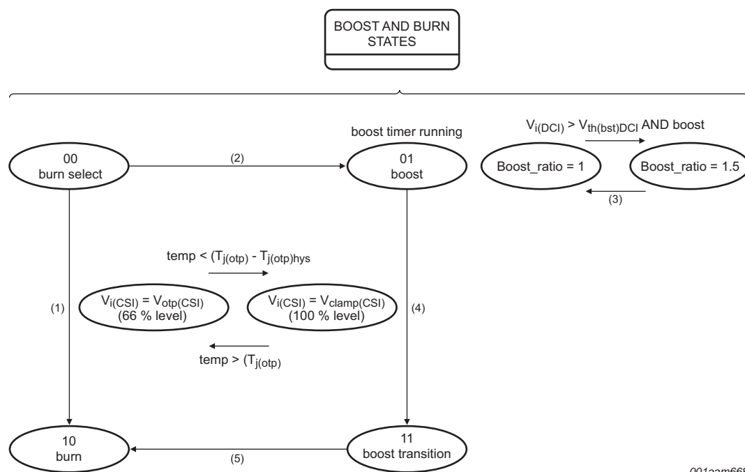
(1) Temp > T_{j(bp)bst} OR Boost_Disable (2) Temp < T_{j(bp)bst} AND NOT Boost_Disable (3) NOT (Boost OR Boost transition) (4) Temp > T_{j(end)bst} OR Boost timer ended OR ( Boost\_ratio = 1.5 AND V_{DCI} < V_{th(bst)DCI} - V_{th(bst)hys(DCI)} ) (5) Boost_Transition timer ended OR V_{DCI} < V_{th(bst)DCI} - V_{th(bst)hys(DCI)} OR Temp > T_{j(otp)}
