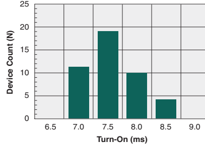
Typical Turn-On Time (N=50, I_F=10\text{mA} , I_L=1\text{A}_{DC} )
