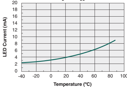
Typical I_F for Switch Operation vs. Temperature ( I_L=0.5\text{A}_{DC} )
