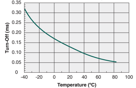
Typical Turn-Off Time vs. Temperature ( I_F=10\text{mA} , I_L=0.5\text{A}_{DC} )
