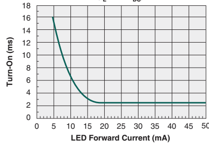
Typical Turn-On Time vs. LED Forward Current ( I_L=0.5\text{A}_{DC} )
