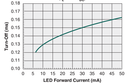
Typical Turn-Off Time vs. LED Forward Current ( I_L=0.5\text{A}_{DC} )
