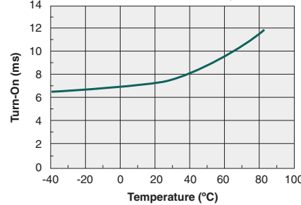
Typical Turn-On Time vs. Temperature ( I_F=10\text{mA} , I_L=0.5\text{A}_{DC} )
