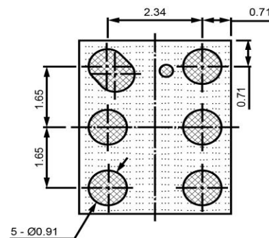
BOTTOM VIEW (1)
