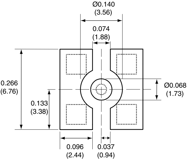
RECOMMENDED FOOTPRINT
