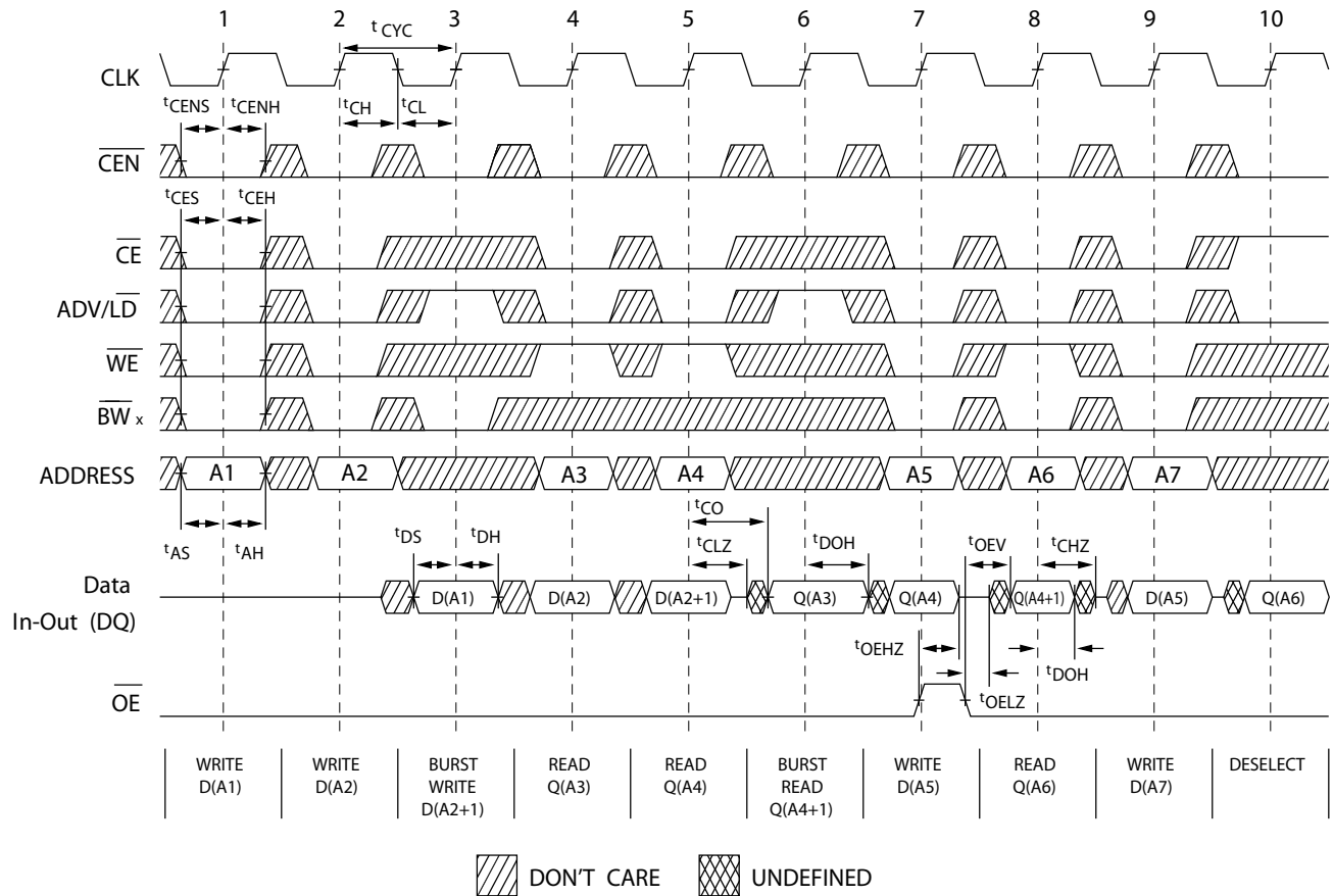
Figure 5. Read/Write/Timing [33, 34, 35]
