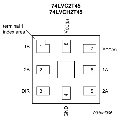
Fig 6. Pin configuration SOT902-2
