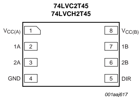
Fig 5. Pin configuration SOT996-2
