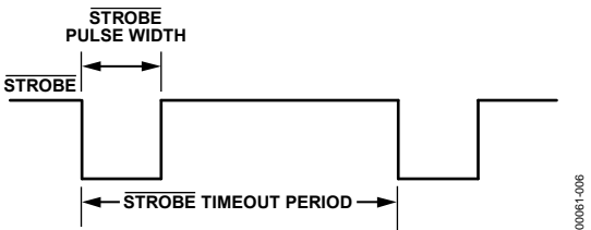
Figure 6. \overline{\text{STROBE}} Parameters
