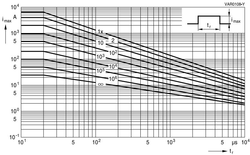
SIOV-S20K510 ... K1000
