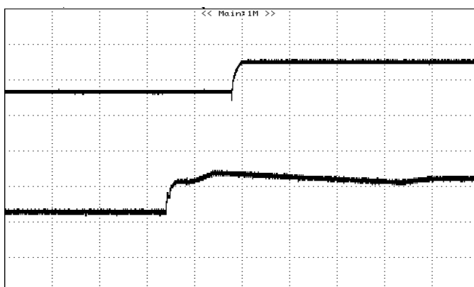
Figure 18: Turn on with Prebias 12Vin, 5V/0A out, Vbias =3.3Vdc . (5mS/div)
