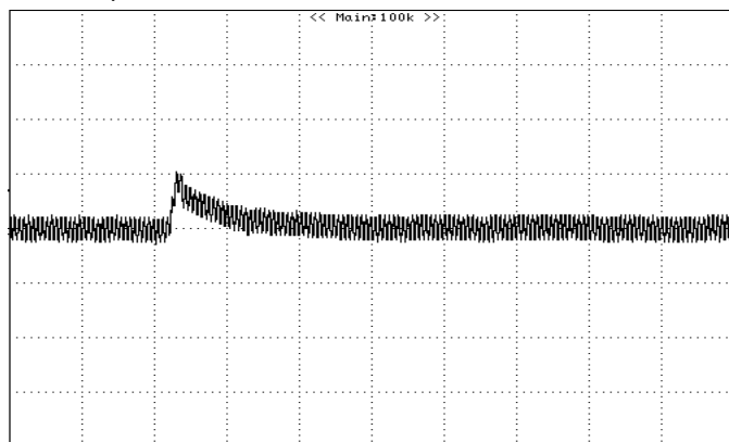
Figure 15: Typical transient response to step load change at 2.5A/ \mu S from 100% to 50% of I_o , max at 12Vin, 5.0V out ( C_{out} = 1\mu F ceramic+ 47 \mu F Ceramic)(100mV/div, 50 \mu S /div)
