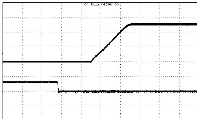
Figure 14: Turn on Using Remote On/Off with external capacitors ( C_o= 3000 \mu F ), 5.0V/3A out(resistive load)(2mS/div)
