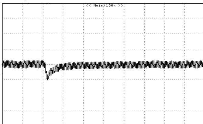
Figure 16: Typical transient response to step load change at 2.5A/ \mu S from 50% to 100% of I_o , max at 12Vin, 5.0V out ( C_{out} = 1\mu F ceramic+ 47 \mu F Ceramic)(100mV/div, 50 \mu S /div)
