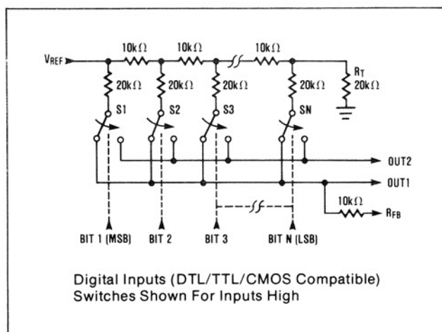
Figure 1. MX7541A Functional Diagram
