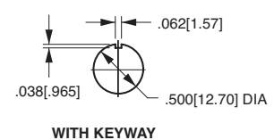
WITH KEYWAY
