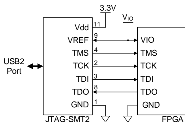
Figure 1. JTAG-SMT2 port connections.
