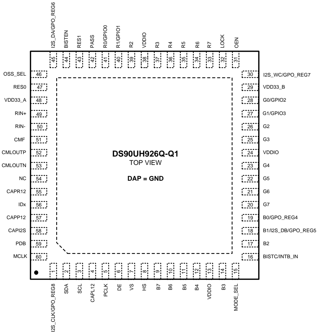
Pin Functions
