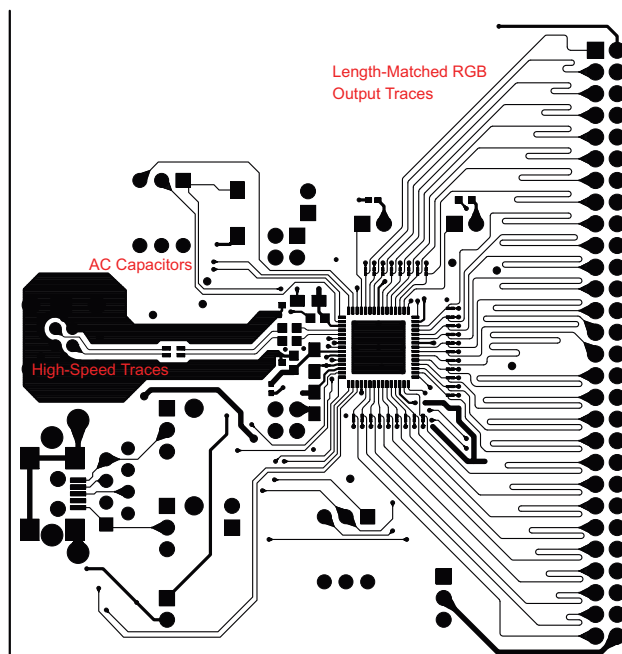
Figure 28. DS90UH926Q-Q1 Deserializer Example Layout
