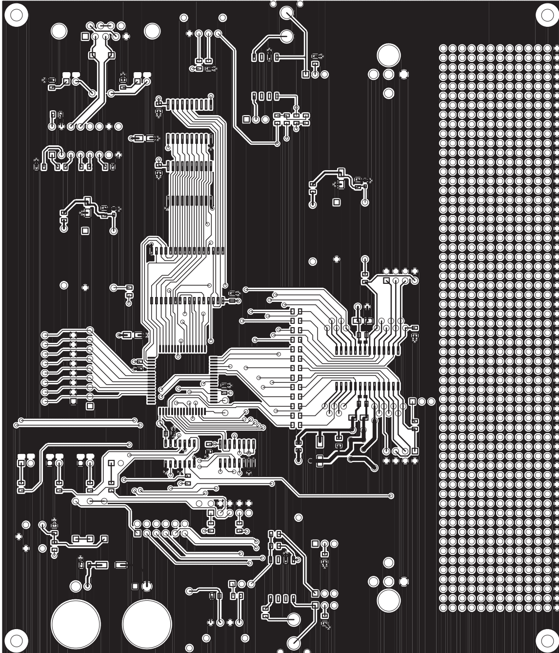
Figure 7. Top PCB
