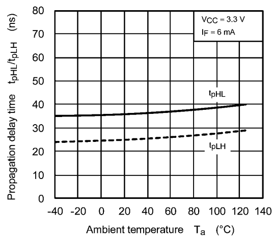
Fig. 12.2.9 t_{pHL}/t_{pLH} - T_a
