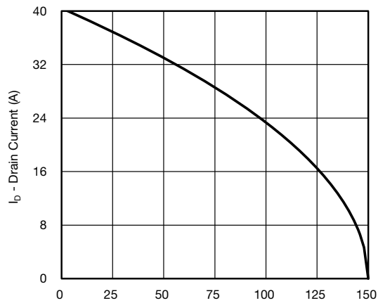
Current Derating*
