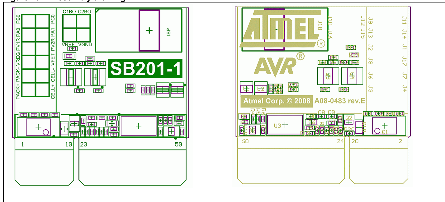
Figure 10-1. Assembly drawing.
