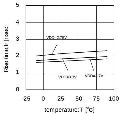
Fig.85 78MHz Rise-time
