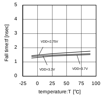
Fig.86 78MHz Fall-time
