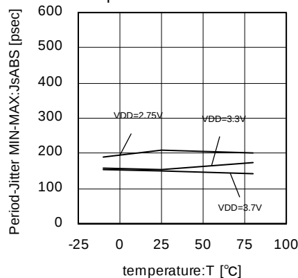
Fig.88 78MHz Jitter-MinMax
