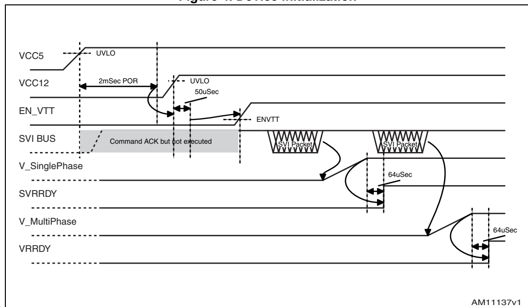
Figure 4. Device initialization
