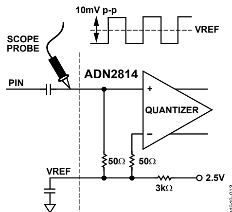
Figure 13. Single-Ended Sensitivity Measurement
