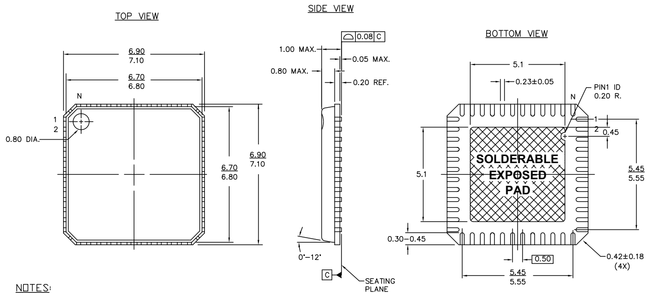
Figure 10-2. 48-Pin (7 × 7 mm) QFN
