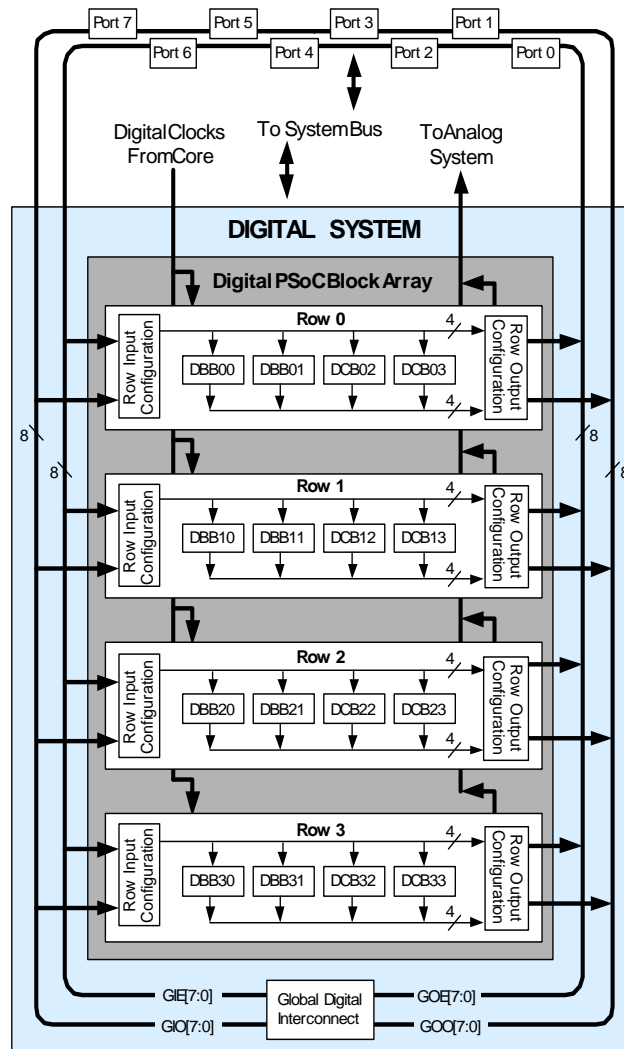
Figure 3-3. Digital System Block Diagram
