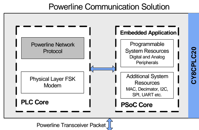
Figure 2-3. Powerline Network Protocol
