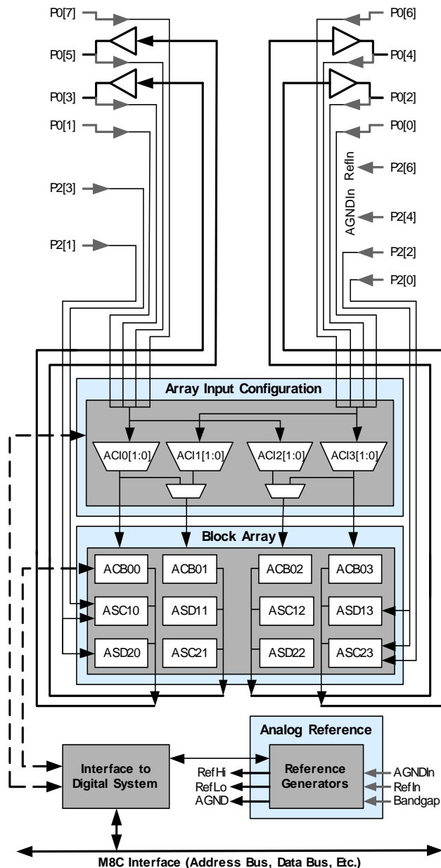
Figure 3-4. Analog System Block Diagram
