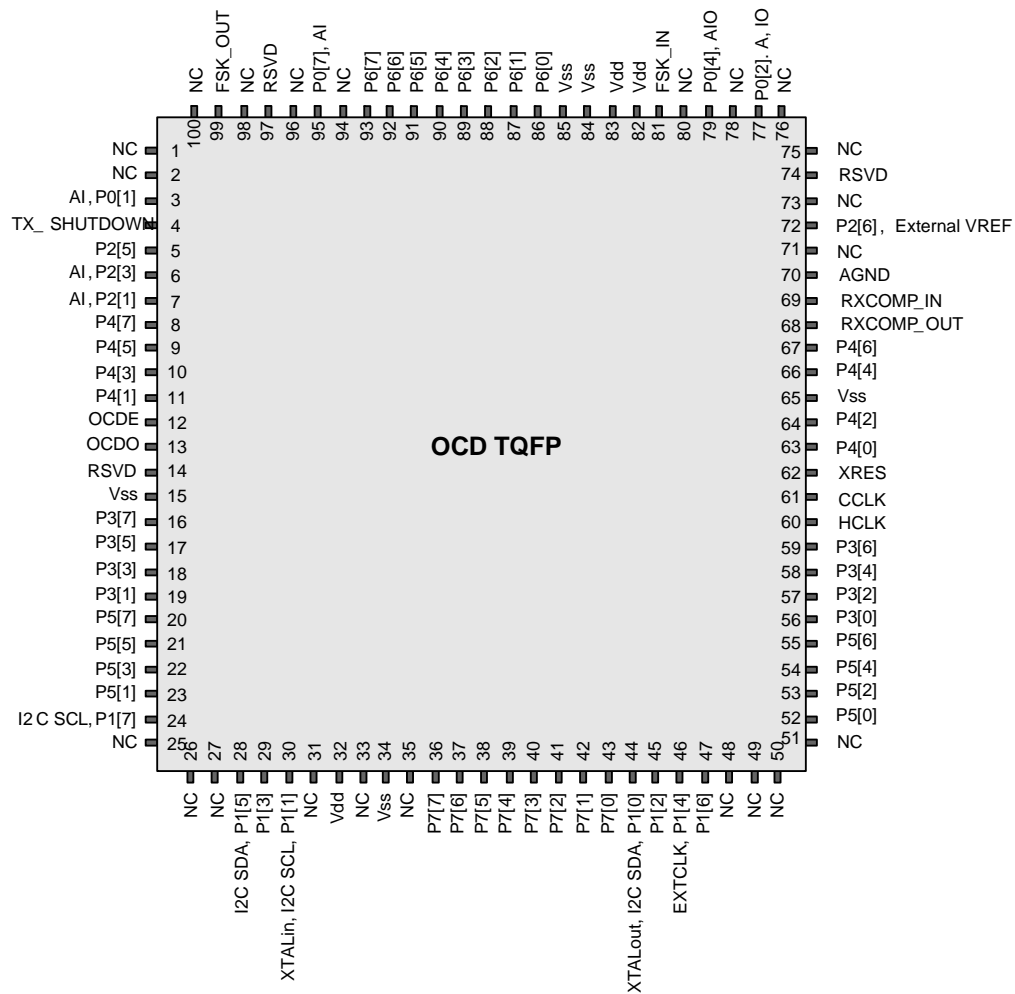
Figure 7-3. CY8CPLC20-OCD
