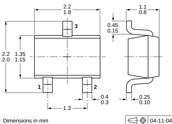
Fig 15. Package outline PDTC114YU (SOT323/SC-70)
