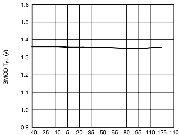
Temperature (°C) SMOD Falling Threshold (V) vs. Temperature (°C) V_{CIN} = V_{DRV} = 5\text{ V}
