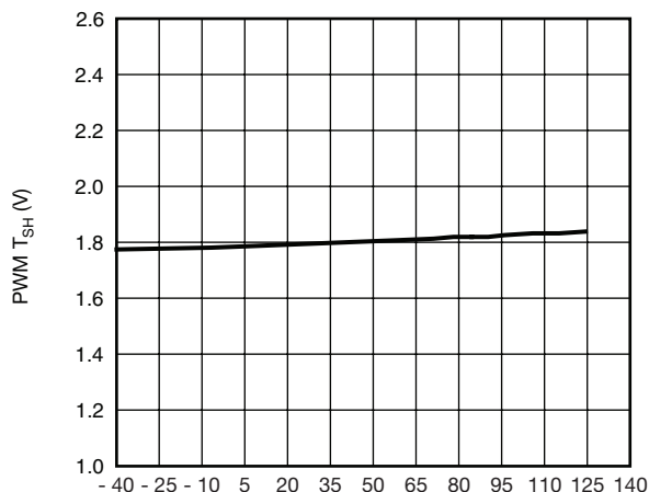
Temperature (°C) PWM Falling Tristate (V) vs. Temperature (°C) V_{CIN} = V_{DRV} = 5\text{ V}
