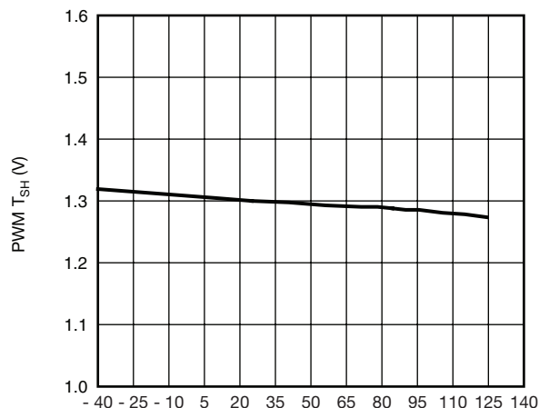
Temperature (°C) PWM Rising Tristate Threshold (V) vs. Temperature (°C) V_{CIN} = V_{DRV} = 5\text{ V}
