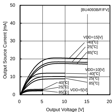
Fig.41 Output sink current—voltage characteristics
