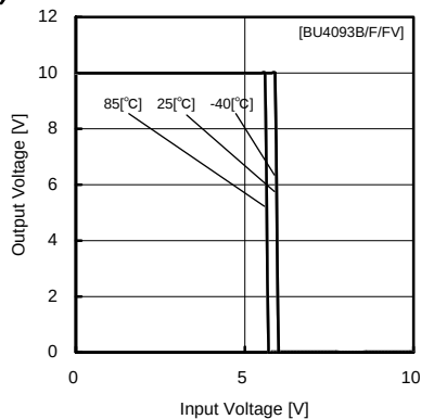
Fig.38 Output voltage—Input voltage characteristics (VDD=10[V] / VSS=0[V])
