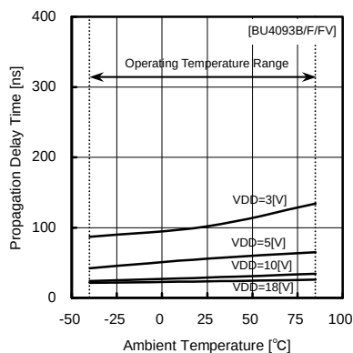
Fig.44 Rising propagation delay tPLH
