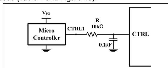
Figure 19 AGC1 Mode Circuit
