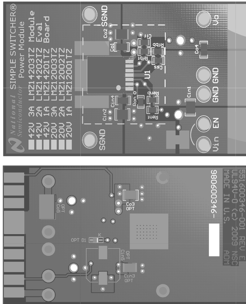
Figure 41. Top And Bottom View Of Evaluation PCB
