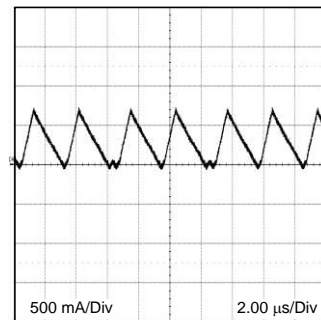
Figure 39. Transition Mode Operation V_{IN} = 12V , V_O = 3.3V , I_O = 0.29A 2 \mu\text{sec/div}
