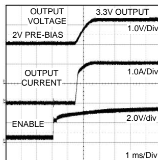
Figure 40. Pre-Biased Startup
