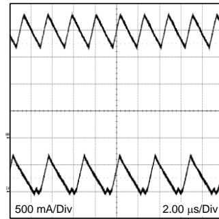
Figure 38. CCM and DCM Operating Modes V_{IN} = 12V , V_O = 3.3V , I_O = 2A/0.26A 2 \mu\text{sec/div}
