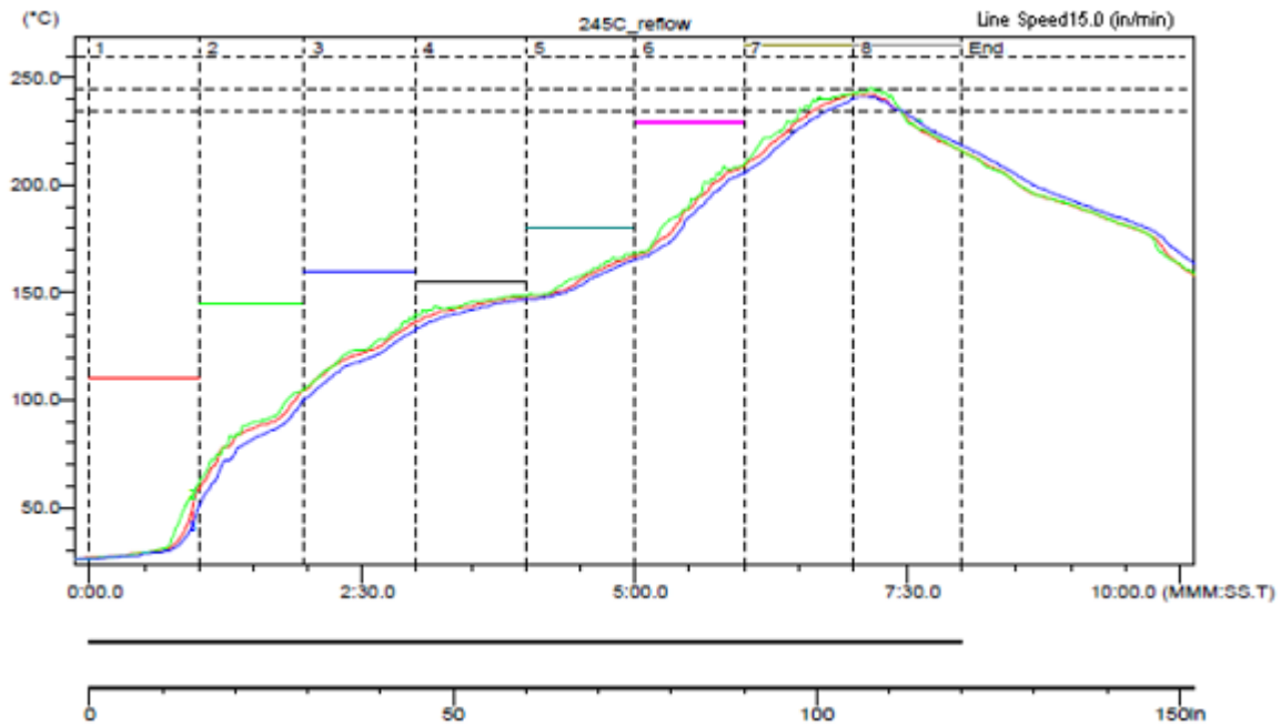
Figure 42. Sample Reflow Profile
