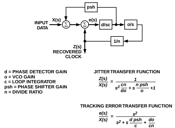
Figure 13. PLL/DLL Architecture
