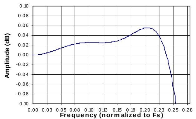
Figure 12. Quad-Speed Passband Ripple
