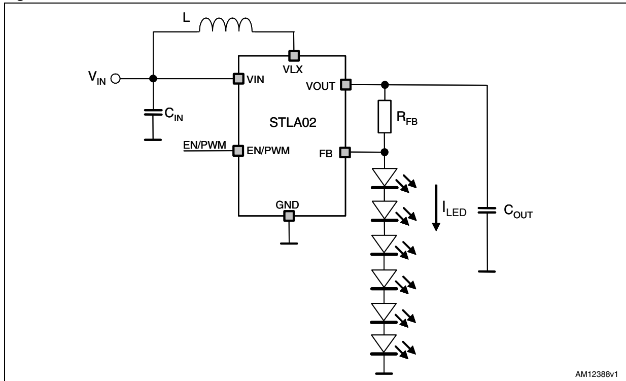
Figure 1. Schematic
