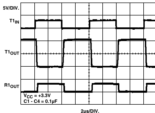
FIGURE 14. ISL4238E/ISL4244E LOOPBACK TEST AT 250kbps ( C_L = 1000\text{pF} )
