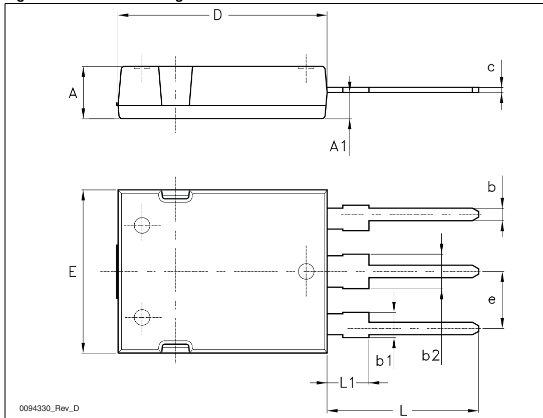
Figure 20. Max247 drawing
