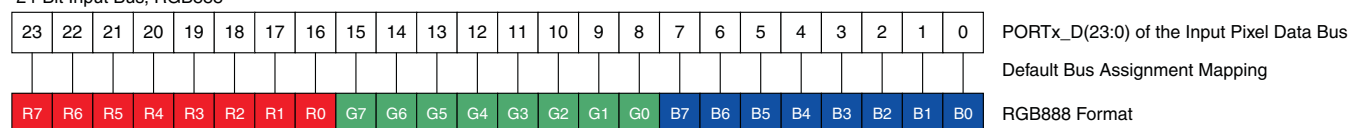
Figure 13. Pixel Mapping
