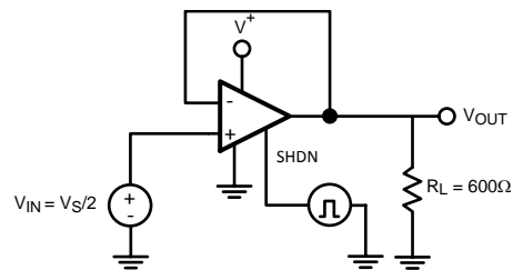
Figure 49. Turn-off Time
