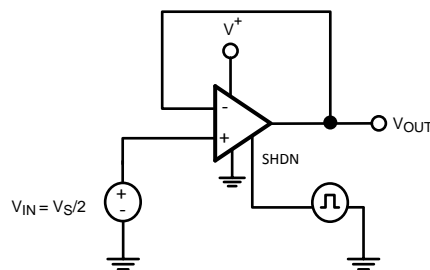
Figure 48. Turn-on Time
