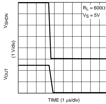
Figure 47. Turn-off Time
