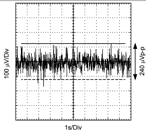
Figure 26. 0.1–10 Hz Noise
