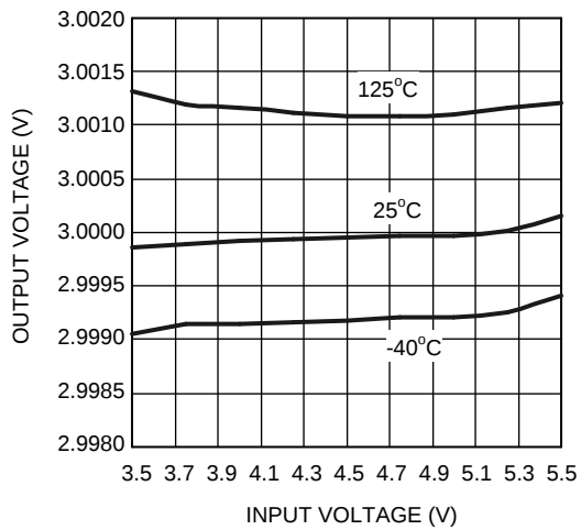
Figure 31. Line Regulation
