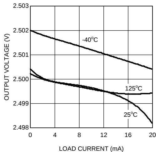
Figure 24. Load Regulation
