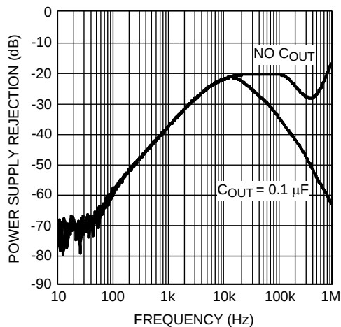
Figure 40. Power Supply Rejection vs Frequency
