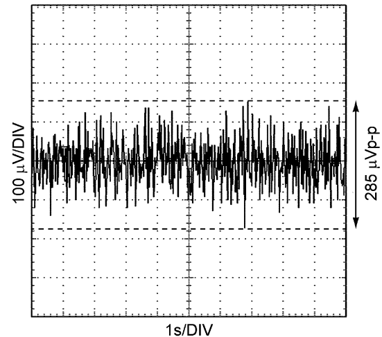
Figure 32. 0.1–10 Hz Noise
