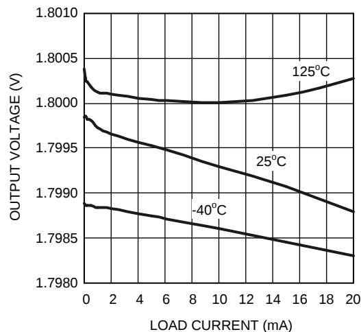
Figure 12. Load Regulation
