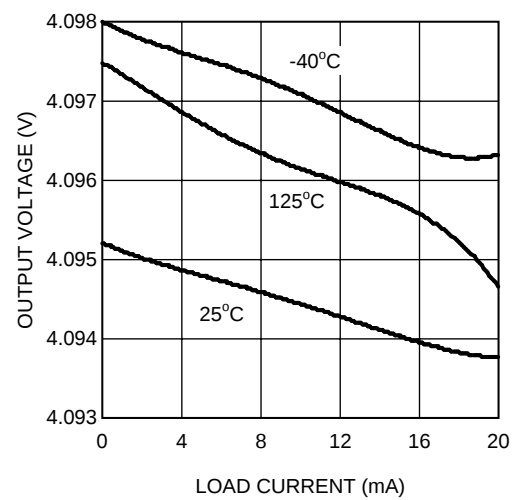
Figure 42. Load Regulation
