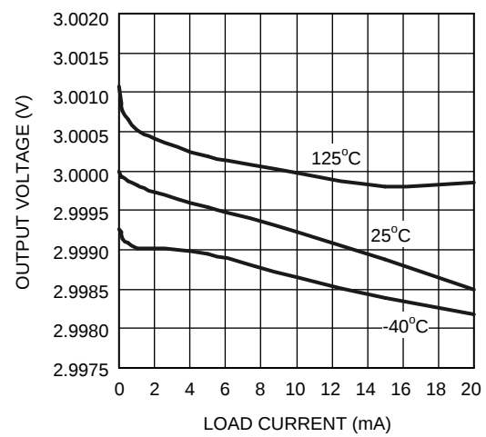
Figure 30. Load Regulation
