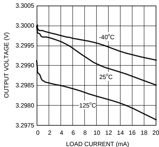
Figure 36. Load Regulation
