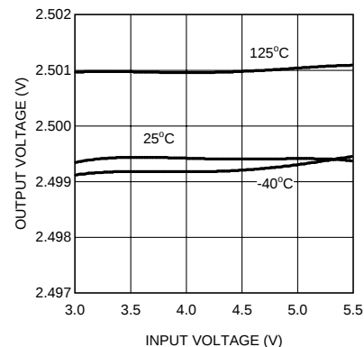
Figure 50. Line Regulation
