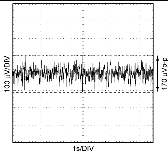
Figure 14. 0.1–10 Hz Noise
