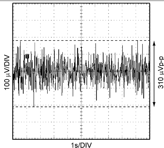
Figure 38. 0.1–10 Hz Noise
