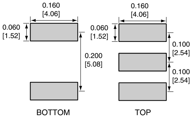
RECOMMENDED FOOTPRINT
