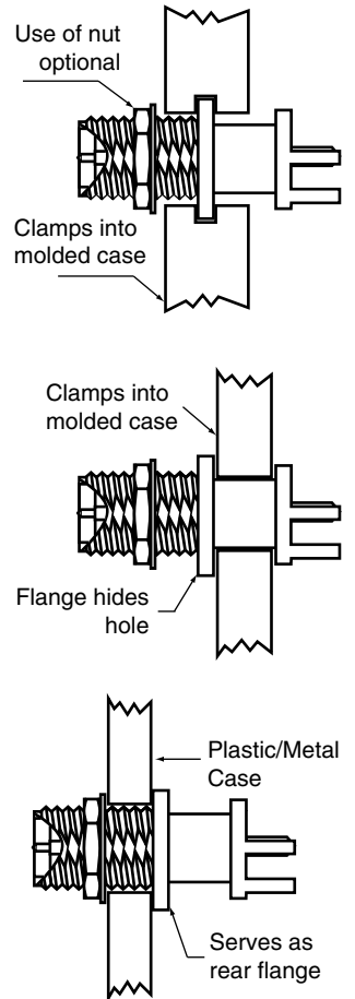
MOUNTING METHODS
