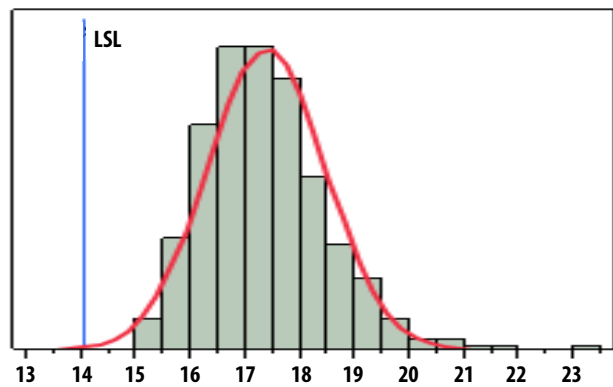
Figure 4. IIP3, LSL = 14 dBm, nominal = 17.3 dBm
