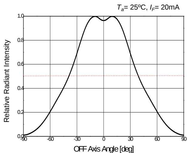
Directivity
