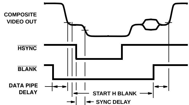
FIGURE 15. HSYNC, BLANK, AND OUTPUT VIDEO TIMING, NORMAL MODE
