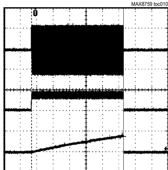
OPEN-LAMP VOLTAGE LIMITING AND TIMEOUT
