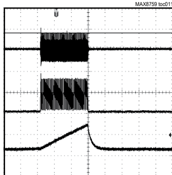
SECONDARY SHORT-CIRCUIT PROTECTION AND TIMEOUT
