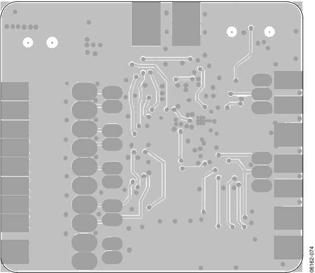
Figure 45. Mirrored Bottom Layers
