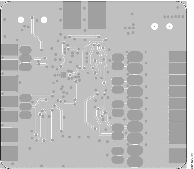
Figure 44. Bottom Layers
