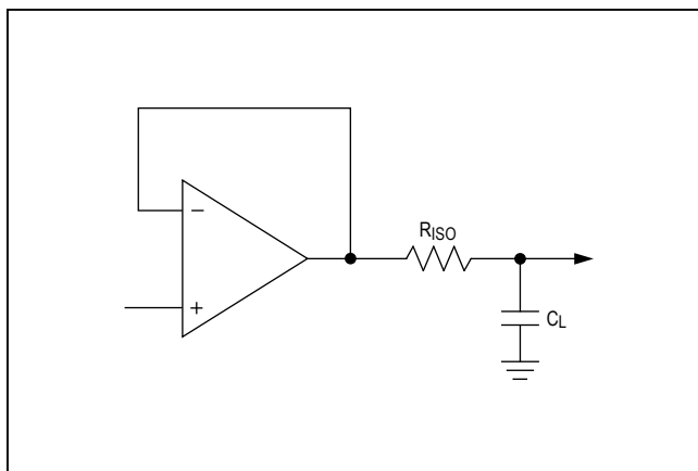
Figure 9. Capacitive-Load-Driving Circuit
