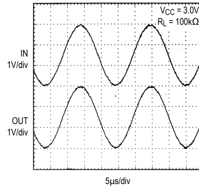
Figure 4. Rail-to-Rail Input/Output Range
