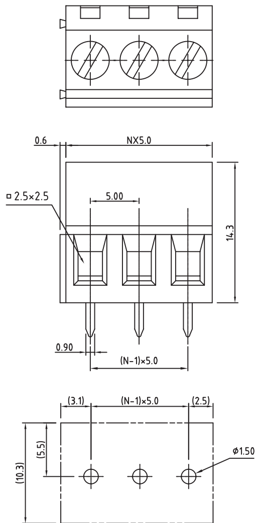
PCB LAYOUT - COMPONENT VIEW
