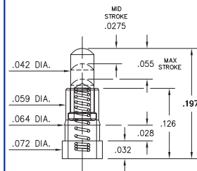
0934-0-15-20-74-14-26-0 Standard Stroke Surface mount
