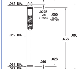
0905-0-00-00-00-00-11-0 Standard Stroke, Surface mount Highest Profile
