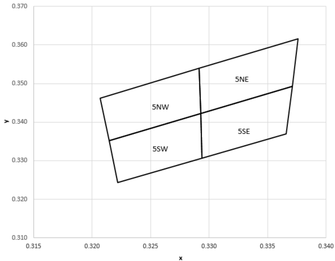
Figure 3C. CIE1931 chromaticity diagram (ANSI standard C78.377-2008)
