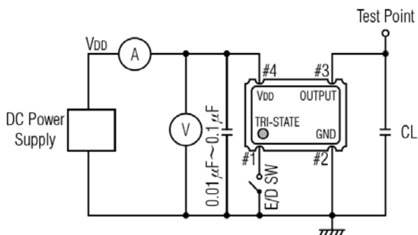
Figure 1) Test Circuit
