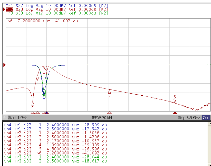
Fig. 3 Frequency Characteristics
