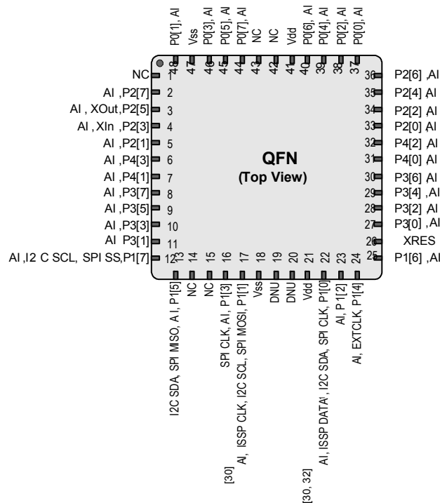
Figure 10. CY8C20636A
