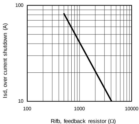
Figure 11 – Ids (A) Vs Rf1b (Ω)
