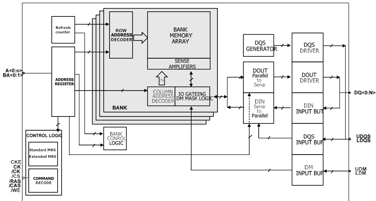
Figure.2 — Block Diagram
