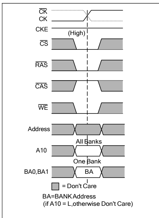
Figure 32 — Precharge command
