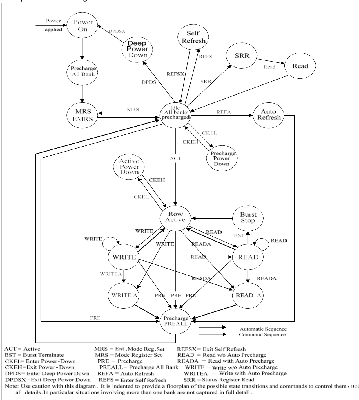
Figure.3 — State Diagram
