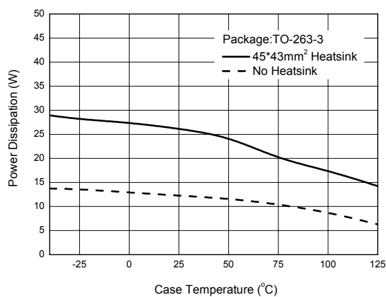
Figure 22. Power Dissipation vs. Case Temperature
